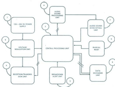
Figure 1: Block diagram of the ADSL receiver system
